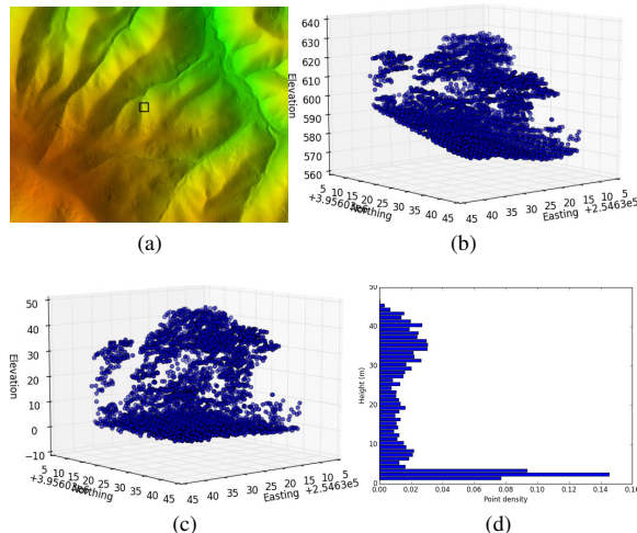
Fig. 3. (a) 3-D LiDAR point cloud at 30 m \times 30 m region (black square) in a typical GSMNP cove forest. (b) The raw LiDAR point cloud (3,985 points), showing the imprints of the underlying cove topography. (c) LiDAR point cloud after topographic detrending and filtering (3,936 points) that converted the elevations to above ground level elevation. (d) Distribution of LiDAR point density along the vertical profiles in a cove forest dominated by tall trees and a dense understory.
