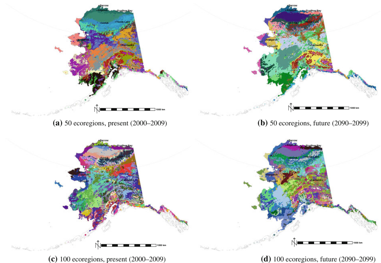
Fig. 2 The 50 ( a and b ) and 100 ( c and d ) most-different quantitatively defined ecoregions for the State of Alaska in the present ( a and c ) and future ( b and d ) decades were derived from 37 variables and are shown using random colors . Realized
