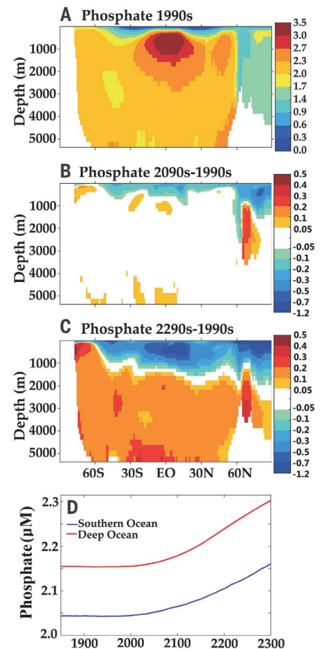
Fig. 4. Southern Ocean nutrient trapping transfers phosphate to the deep ocean. Zonal mean phosphate concentrations (micromolar) are shown for the 1990s (A), along with the differences in zonal phosphate concentrations in comparisons of the 1990s with the 2090s (B) and the 1990s with the 2290s (C). Phosphate concentrations increase over time in the high-latitude Southern Ocean (at all depths south of 60°S) and in the global deep ocean (below 2000 m and north of 60°S) (D).
