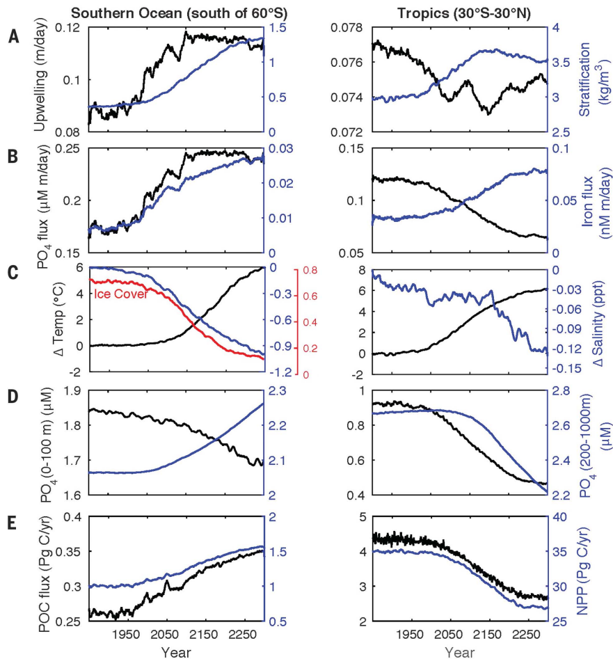
Fig. 3. Regional time series of ocean physical forcing and biogeochemical response.
