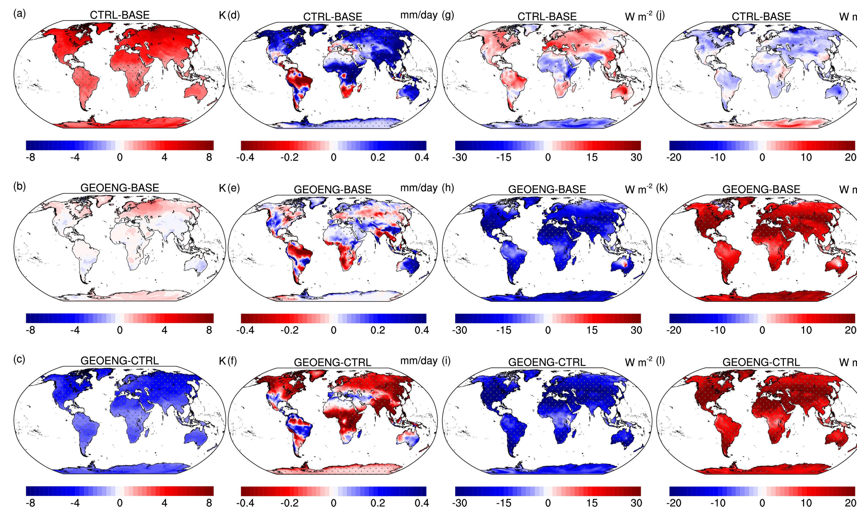
Figure 3: Changes of spatial distributions between CTRL and BASE (top row), between GEOENG and BASE (middle row), and between GEOENG and CTRL (bottom row) for surface temperature (K, (a)–(c)), precipitation (mm day -1 , (d)–(f)), total downward direct solar radiation at the surface (W m -2 , (g)–(i)), and total downward diffuse solar radiation at the surface (W m -2 , (j)–(l)). The spatial distribution of CTRL is from the 2020–2097 time-averaged results without geoengineering while that of GEOENG is from the 2020–2097 time-averaged results with geoengineering applied. The spatial distribution of BASE is from the 2010–2019 time-average results. Light grey stippling (dots) indicates regions where the change is significant using the Student's t-test ( p < 0.1 ).
