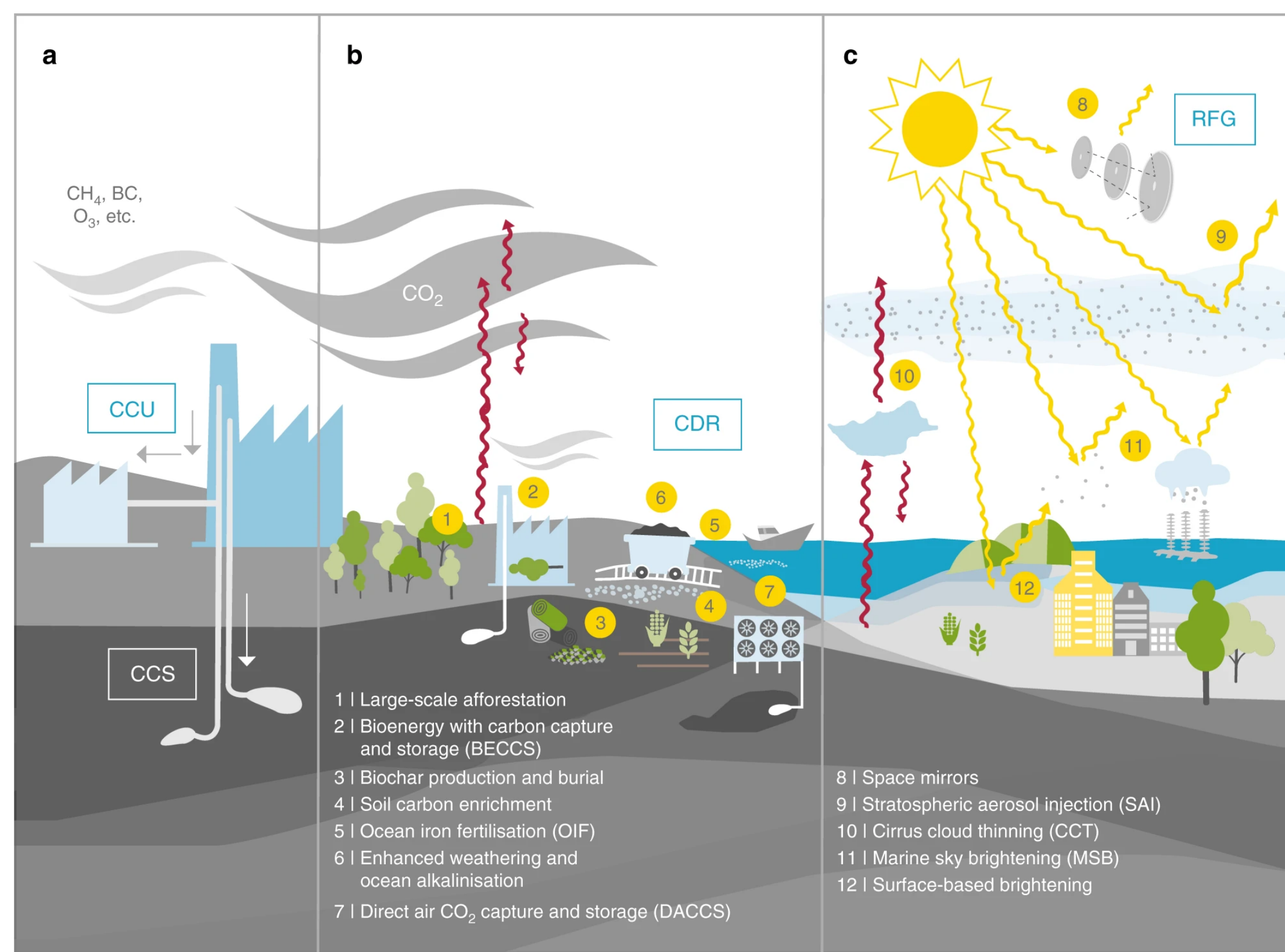
Figure 1: Proposed climate geoengineering techniques placed in the context of mitigation efforts. Adopted from Lawrence et al. (2018).
