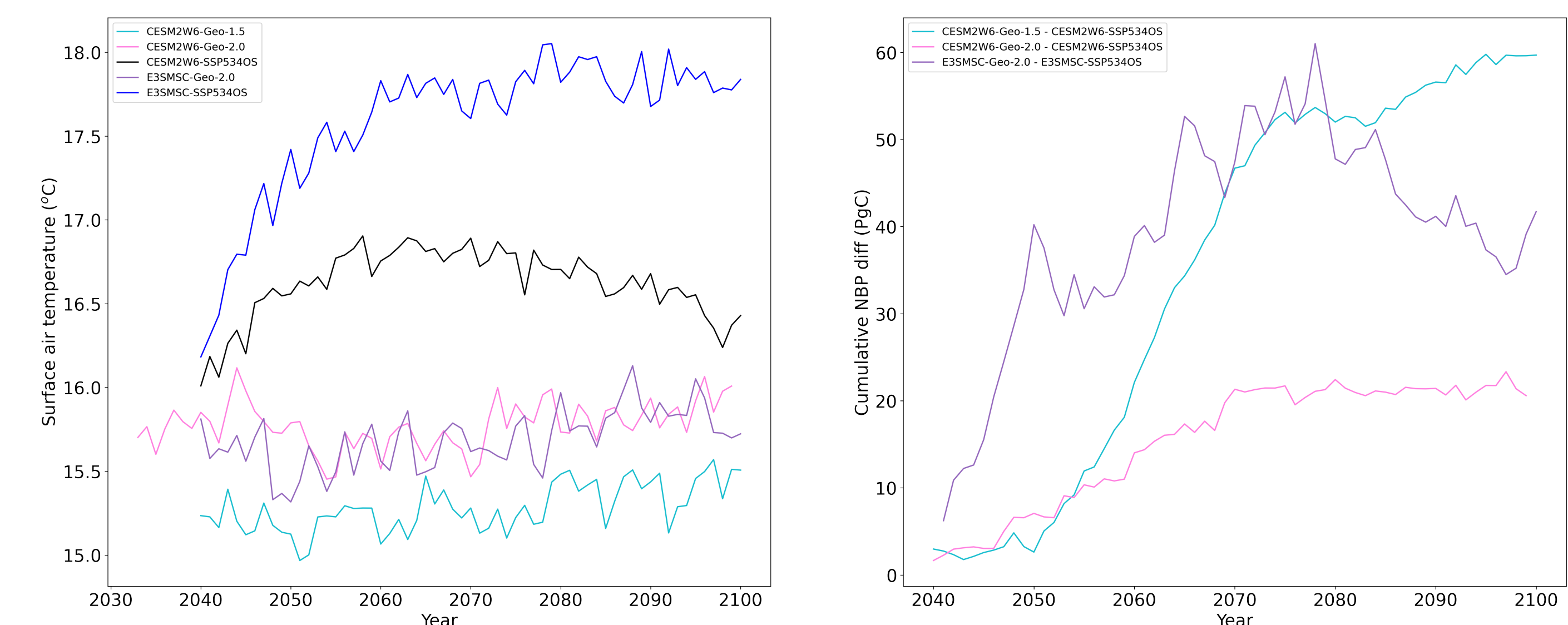
Figure 7: Such "peak shaving" simulations have been performed with the Community Earth System Model version 2 (CESM2) and E3SM. In all simulations, the SSP5-3.4-OS scenario was used, first without SAI then with SAI. CESM2 was used to simulate both 1.5° and 2.0° temperature targets, and E3SM has so far been used to simulate a 2.0° temperature target. (Left) Surface temperature for the baseline SSP5-3.4-OS simulations and a single ensemble member of 1.5° and 2.0° simulations from CESM2 and the 2.0° simulation from E3SM. (Right) The cumulative difference in land carbon storage for the three SAI scenarios represented in the panel on left. In all cases, SAI induced a stronger land carbon sink. By the year 2100, the 1.5° simulation from CESM2 had the largest increase in land carbon storage, the CESM2 2.0° simulation has the smallest increase, and the E3SM 2.0° simulation ended up in between the other two.
