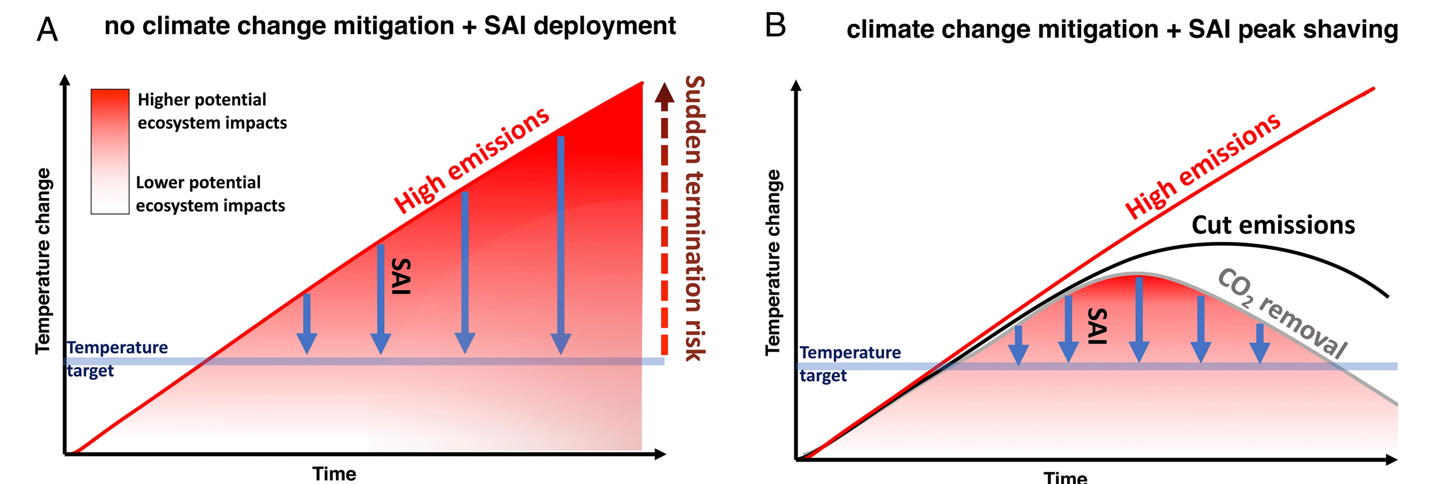
Figure 6: Potential temperature change over time for two different SAI scenarios. (A) In a future with no climate change mitigation and with SAI deployment, high emissions result in rising temperatures (red line). Increasing amounts of SAI would have to be deployed to reduce temperature (blue arrows) to a specific temperature target (blue line). The risk of sudden SAI termination also increases (red arrow). (B) In a future with climate change mitigation and SAI "peak shaving," temperature changes are first reduced by a combination of emissions reductions (black line) and CDR (CO 2 removal, gray line), then further reduced by SAI (blue arrows). Adopted from Zarnetske et al. (2021).
