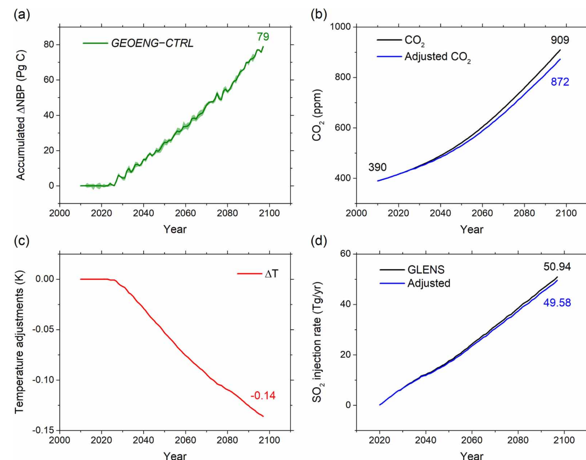
Figure 5: The trajectories of (a) accumulated global carbon sink strength changes (Pg C) due to geoengineering, (b) the atmospheric CO 2 mole fraction (ppm) during 2010–2097 for BASE+CTRL (black line) and the adjusted atmospheric CO 2 mole fraction due to terrestrial BGC feedbacks under geoengineering (blue line), (c) surface temperature responses (K) due to atmospheric CO 2 adjustments, and (d) sulfur injection rates (Tg yr -1 ) in GLENS (red) and adjusted injection rates due to terrestrial BGC feedbacks (blue).
