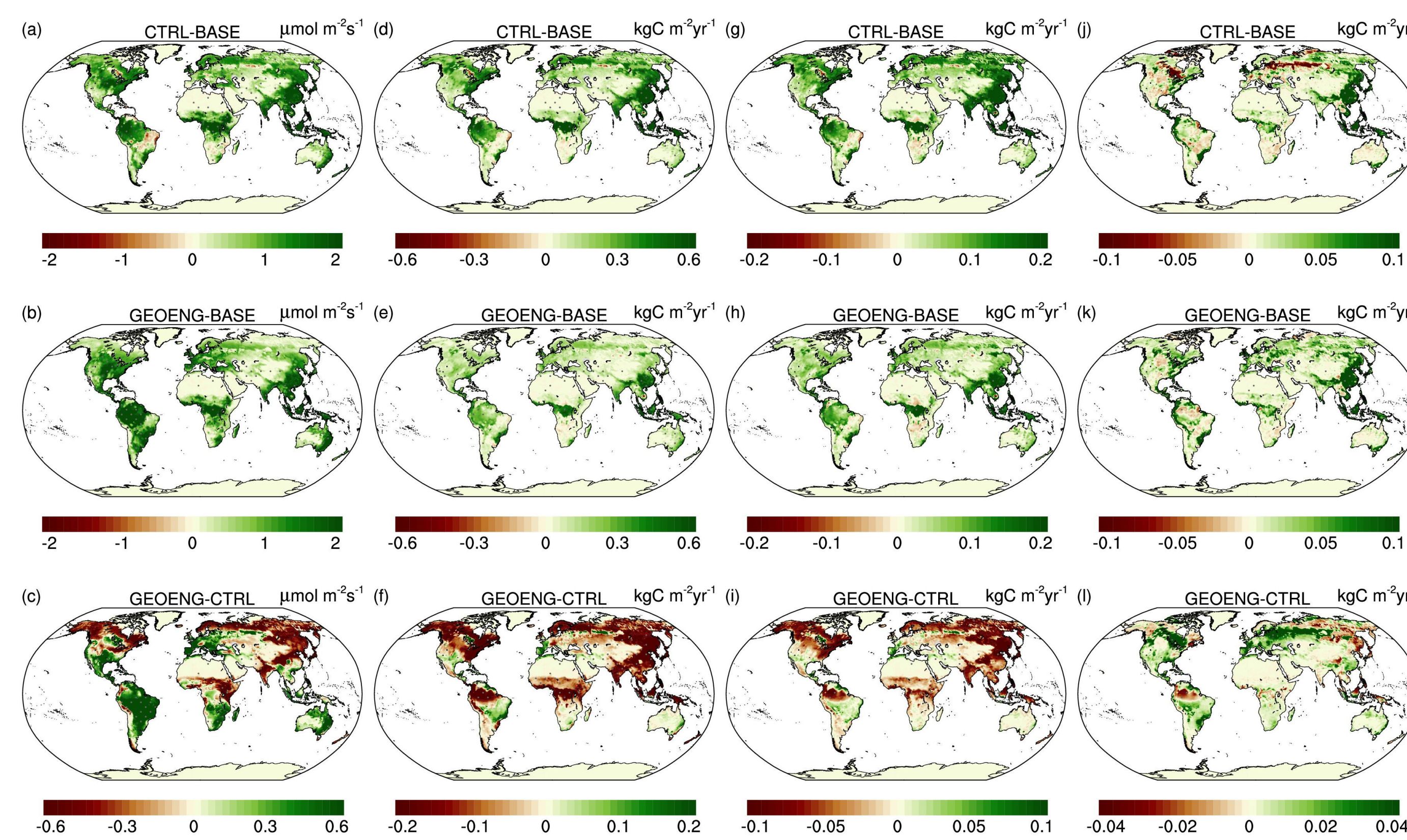
Figure 4: Changes of spatial distributions between CTRL and BASE (top row), between GEOENG and BASE (middle row), and between GEOENG and CTRL (bottom row) for photosynthesis rates ( \mu\text{mol m}^{-2} \text{s}^{-1} , (a)–(c)), gross primary production ( \text{kg C m}^{-2} \text{yr}^{-1} , (d)–(f)), net primary production ( \text{kg C m}^{-2} \text{yr}^{-1} , (g)–(i)), and net biome production ( \text{kg C m}^{-2} \text{yr}^{-1} , (j)–(l)). The spatial distribution of CTRL is from the 2020–2097 time-averaged results without geoengineering while that of GEOENG is from the 2020–2097 time-averaged results with geoengineering applied. The spatial distribution of BASE is from the 2010–2019 time-average results. Light grey stippling (dots) indicates regions where the change is significant using the Student's t-test ( p < 0.1 ).
