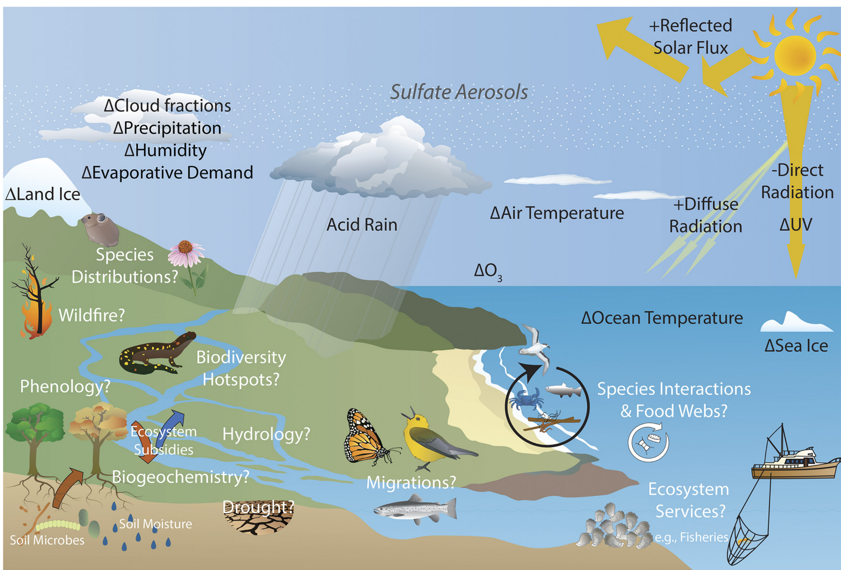
Figure 2: Although some effects of SRM with SAI on the climate are known from certain SAI scenarios (indicated with + for likely increases, - for decreases, Δ to indicate change), the effects of SAI on ecological systems are largely unknown. Adopted from Zarnetske et al. (2021).
