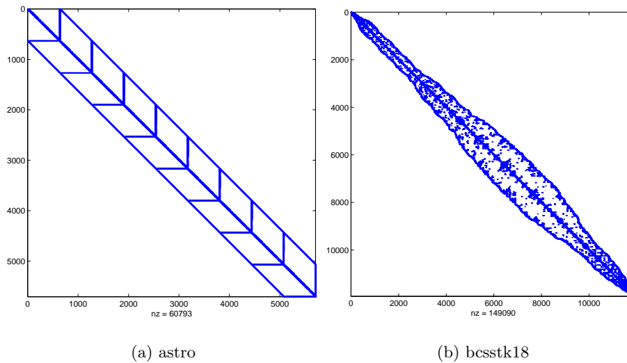
Fig. 7. Sparsity patterns for test matrices
