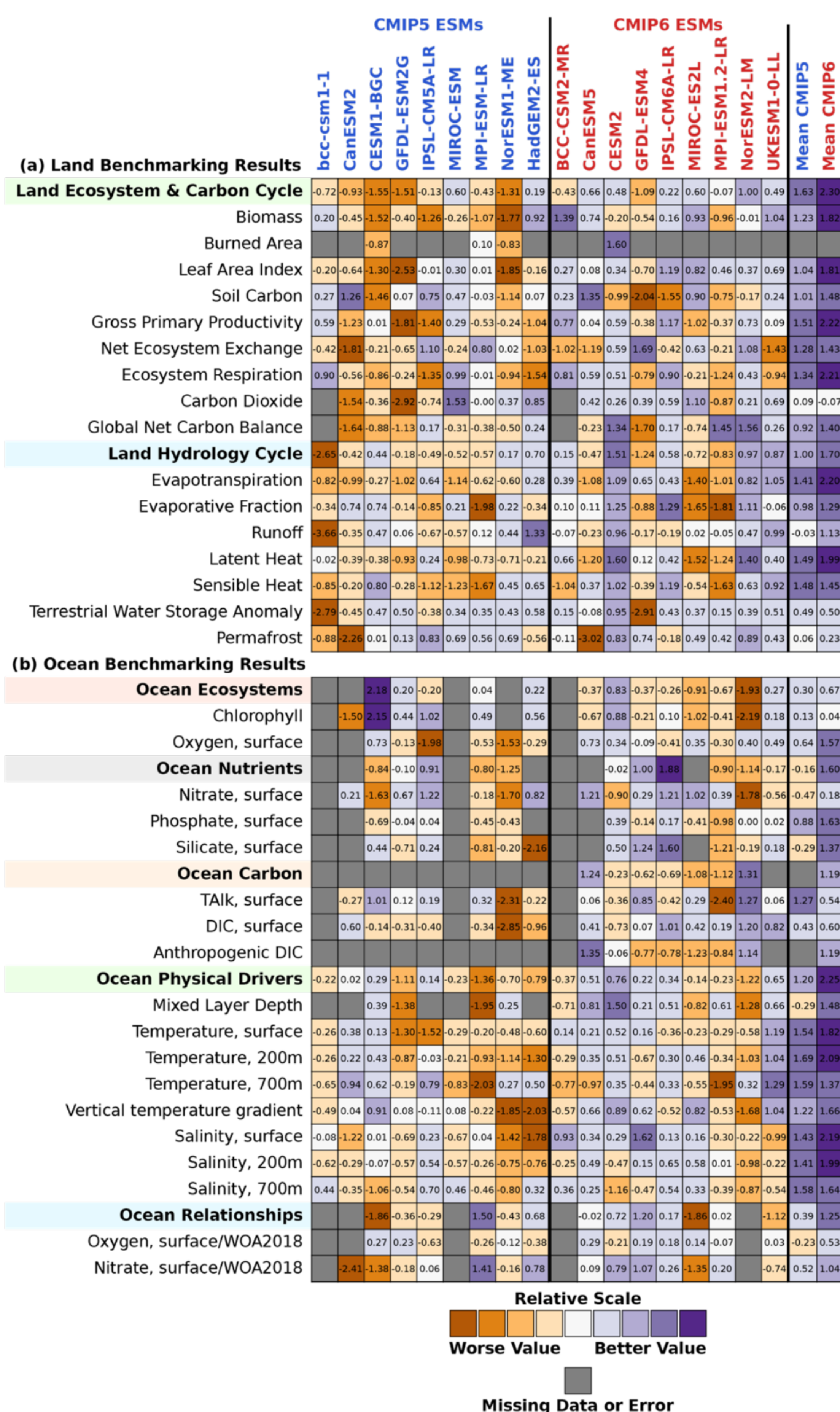
Figure 1: This portrait plot provides an overview of relative scores for CMIP5 (left-hand side of table) and CMIP6 (right-hand side of table) Earth system models (ESMs), for multiple benchmarks against different datasets. (a) Benchmarking of ESM land models from ILAMB; (b) benchmarking of ocean models from the International Ocean Model Benchmarking (IOMB) package. Scores are relative to other models within each benchmark row, with positive scores indicating a better agreement with observations. Models included are only those from institutions that participated in both CMIP5 and CMIP6 carbon cycle experiments, in order to trace changes from one ensemble to the next. CMIP5 models are labels in blue and CMIP6 in red. This is Figure 5.22 in the IPCC Sixth Assessment Report (AR6), Climate Change 2021: The Physical Science Basis.
